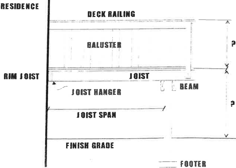
FIGURE 6: FRAMING ELEVATION
