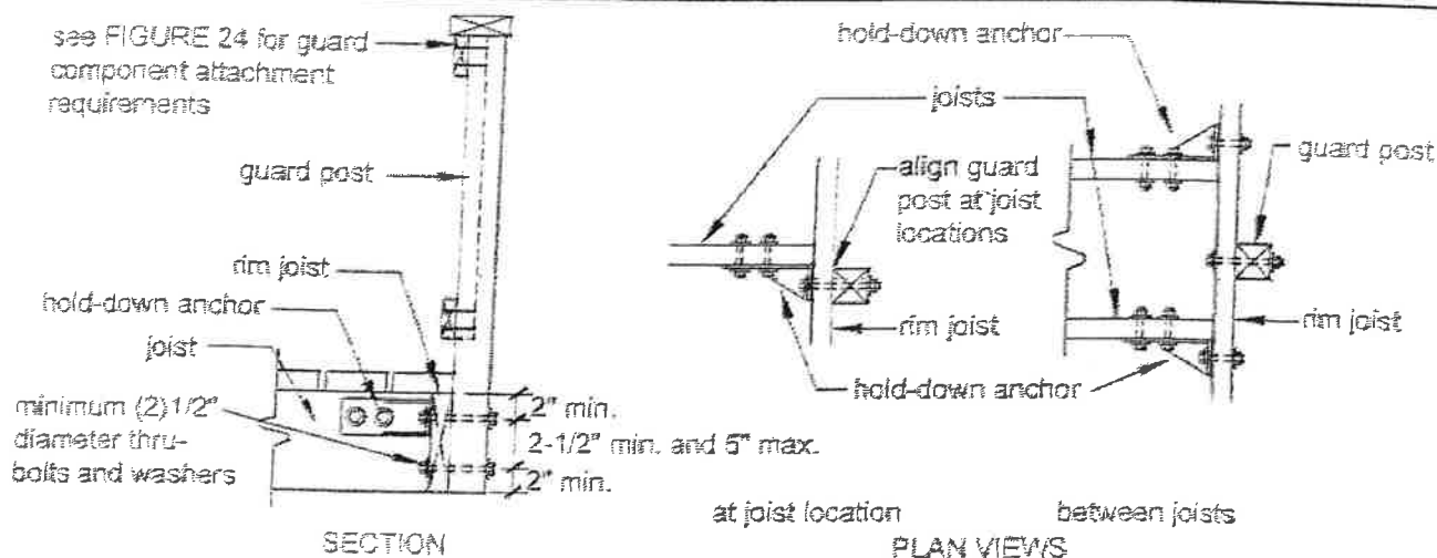
Figure 26. Guard Post to Rim Joist Example
