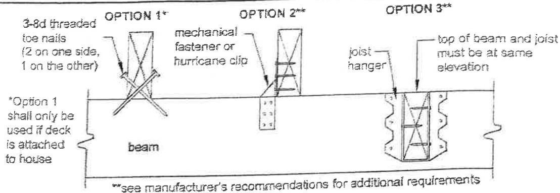
Figure 6: Joist-to-Beam Detail
