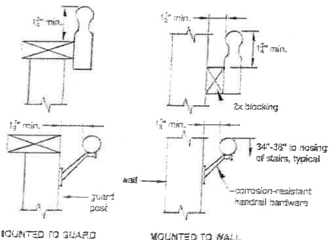
Figure 32A. Handrail Mounting Examples
