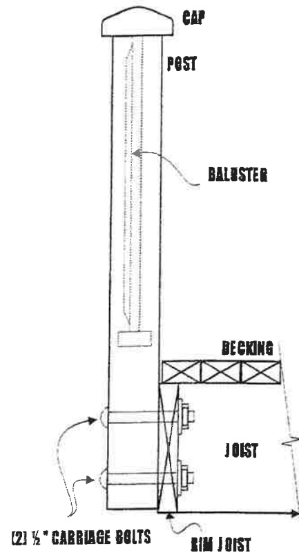
FIGURE 10: DECK RAILING
