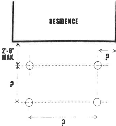
FIGURE 2: FOUNDATION PLAN - FLOATING
