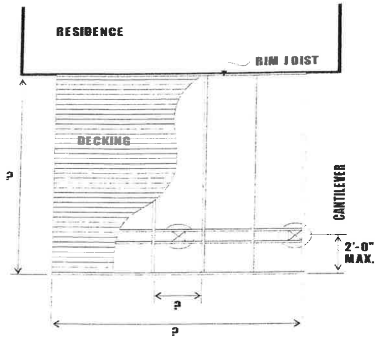
FIGURE 5: FRAMING PLAN
