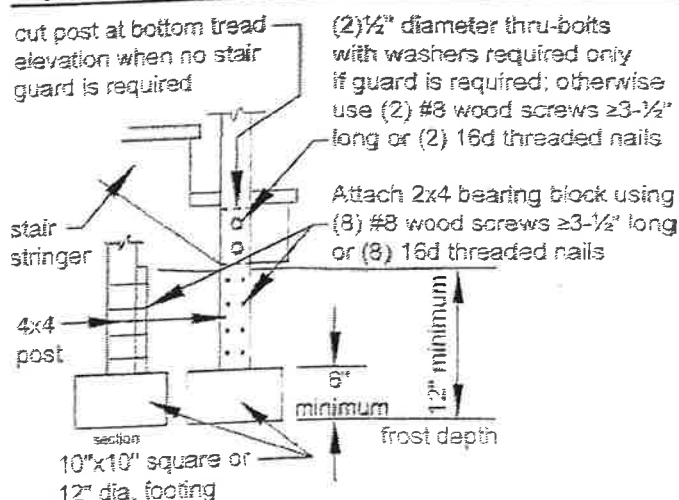
Figure 34. Stair Footing Detail
