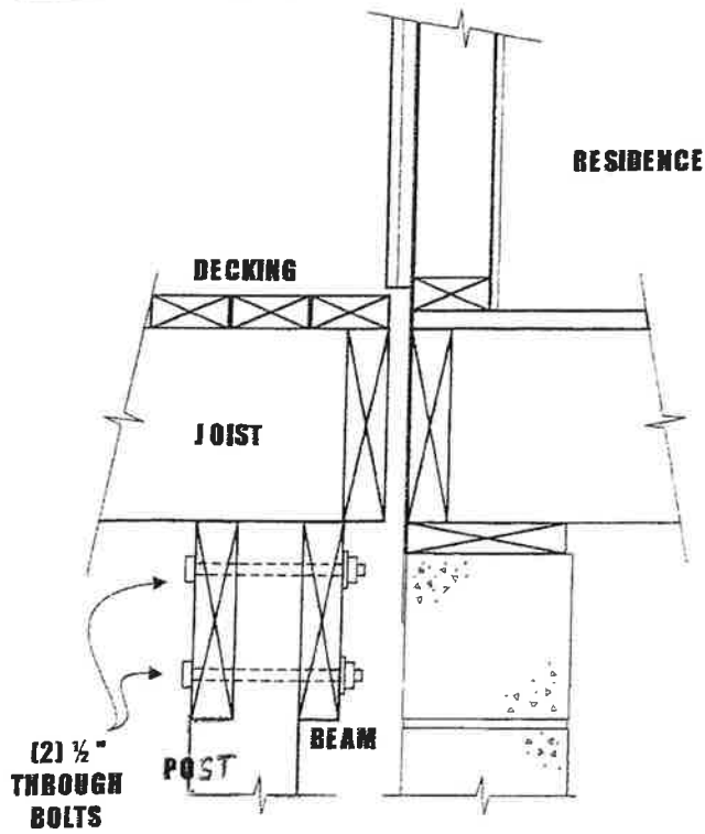
FIGURE 9: FLOATING DECK
