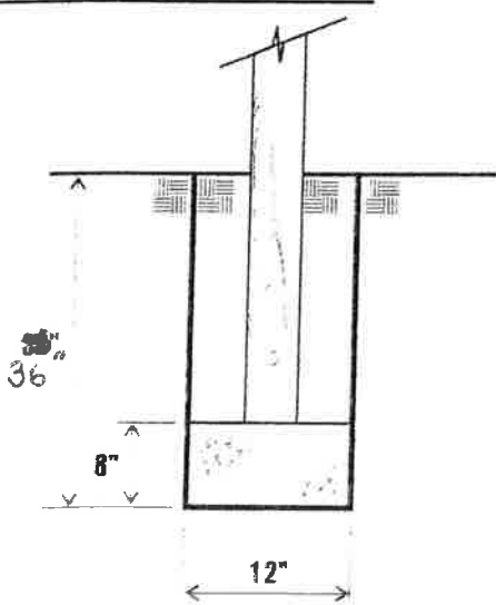
FIGURE 3: FOOTERS - BELOW 72"
