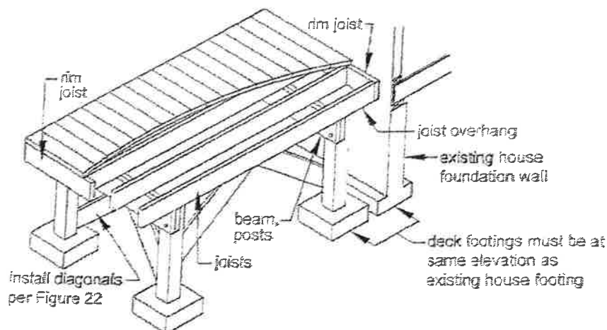
Figure 21. Free-Standing Deck
