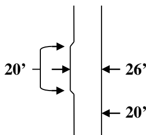
Minimum Clearance Around a Fire Hydrant
