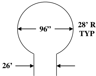
96' Diameter Cul-De-Sac
