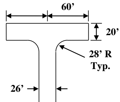
120' Hammerhead
